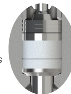
Lower stem does not rotate within the packing preventing seat and stem tip damage and reducing packing wear.
